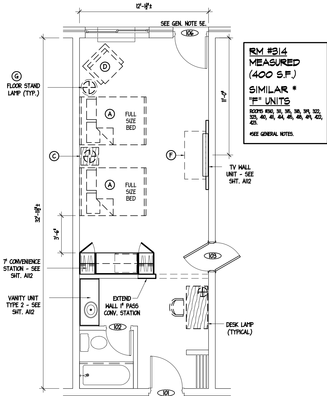
"F" UNIT F2 DBL. FULL BED A103 SCALE: 3/16" = 1'-0"
