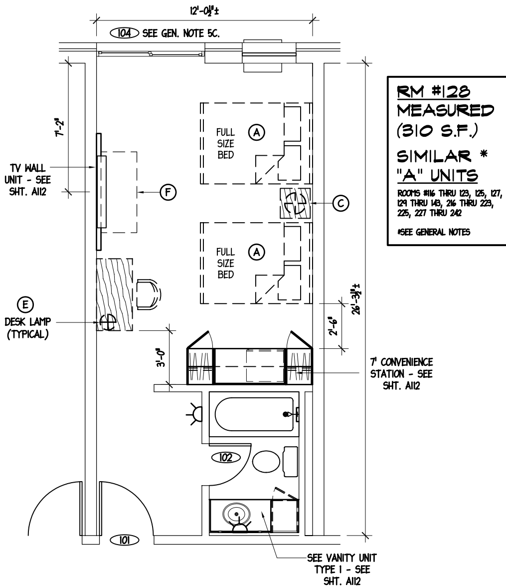
A2 A101 "A" UNIT DBL. FULL BED SCALE: 3/16" = 1'-0"
